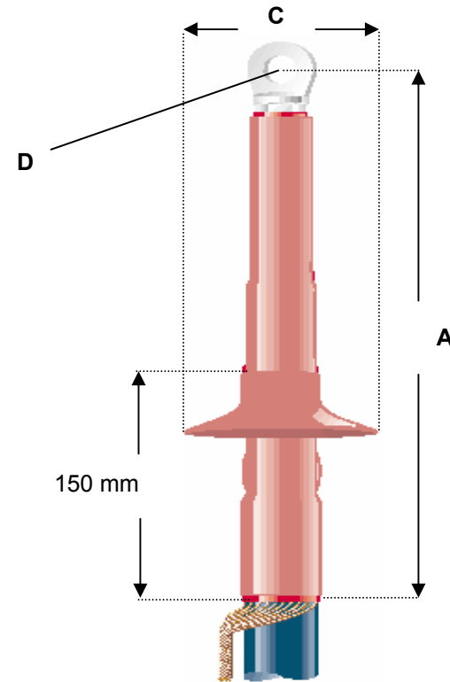
Indoor Termination
