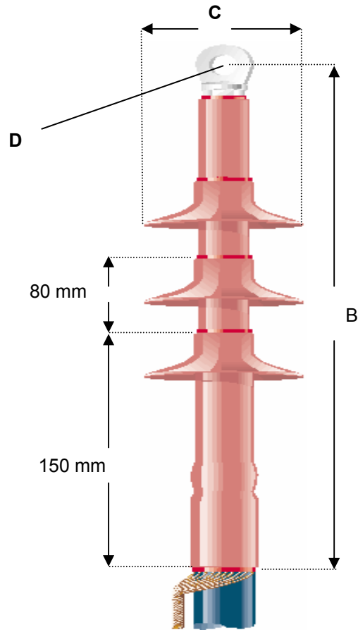
Outdoor Termination
